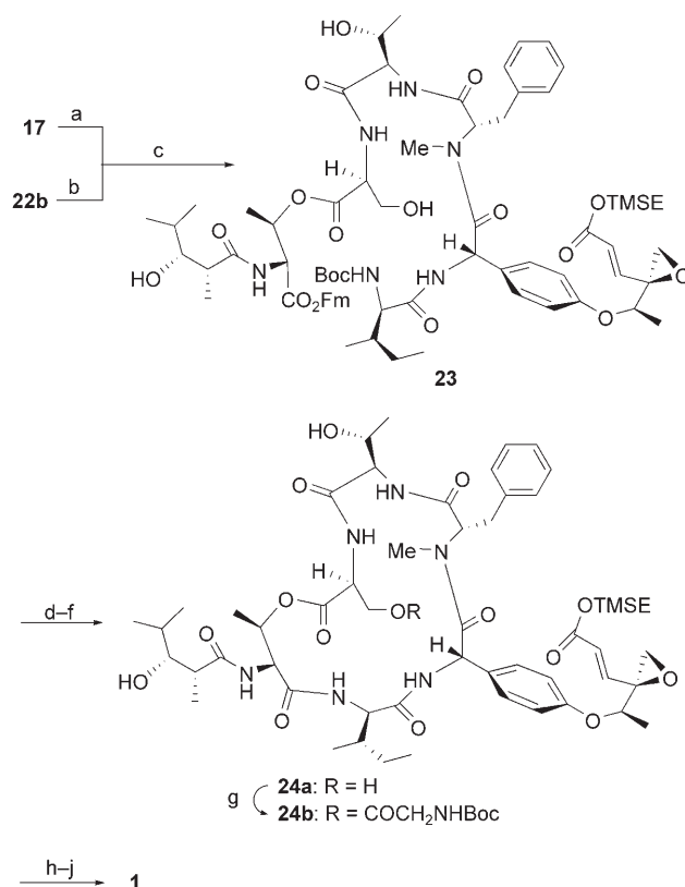
Scheme 5. Reagents and conditions: a) \text{Et}_3\text{N} , THF; b) TFA, \text{CH}_2\text{Cl}_2 ; c) HATU, HOAt, (i\text{Pr})_2\text{NEt} , \text{CH}_2\text{Cl}_2 , DMF, 80% yield from 17; d) \text{HNEt}_2 , \text{MeCN} ; e) TFA; f) HATU, HOAt, (i\text{Pr})_2\text{NEt} , \text{CH}_2\text{Cl}_2 , DMF, 34% yield for 3 steps; g) N-Boc-Gly-OH, EDC, DMAP, 82% yield based on 39% recovery of 23; h) TAS-F, DMF, 87% yield based on 47% recovery of 24b; i) TFA, j) HATU, HOAt, (i\text{Pr})_2\text{NEt} , DMF, 40% yield for 2 steps. TFA = trifluoroacetic acid; TAS-F = tris(dimethylamino)sulfonium difluorotrimethylsilicate.
