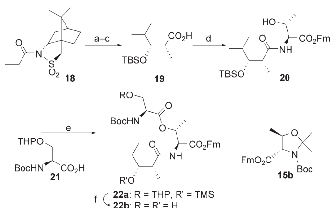
Scheme 4. Reagents and conditions: a) \text{Et}_2\text{BOTf} , (i\text{Pr})_2\text{NEt} , then \text{TiCl}_4 , i\text{PrCHO} ; b) \text{TBSOTf} , 2,6-lutidine, \text{CH}_2\text{Cl}_2 ; c) \text{LiOH} , 30% \text{H}_2\text{O}_2 , THF, 80% yield for 3 steps; d) 15b, \text{HCl} , \text{MeOH} , then 19, HATU, HOAt, (i\text{Pr})_2\text{NEt} , \text{CH}_2\text{Cl}_2 , DMF, 87%; e) 21, EDC, DMAP, \text{CH}_2\text{Cl}_2 , -5^\circ\text{C} , 80%; f) PPTS, \text{MeOH} , 90%.
